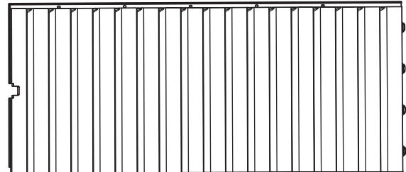
AHD (x1) Wall Panel
